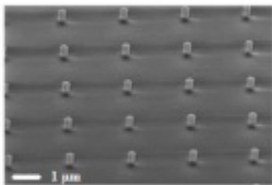
SEM images of AlGaAs nanodisks after oxidation of bottom AlAs layer © 2017 Erganeo
